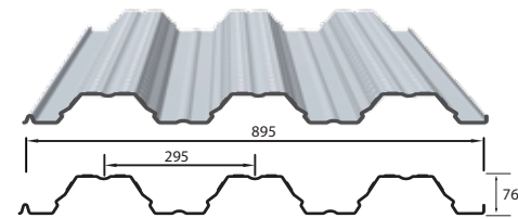
NordicDek® 76
