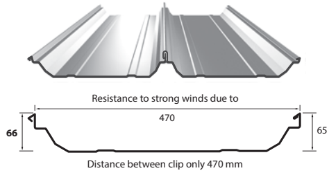
* NordicLok® - for Roof Panel
