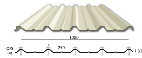
* NordicRoof™ - for Roof Panel
