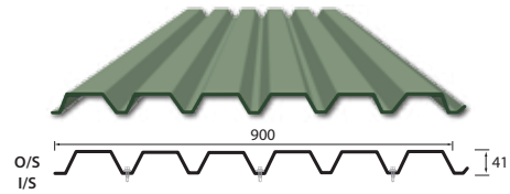
* NordicWall™ - for Wall Panel
