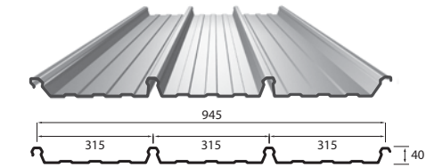
* NordicLok® - for Roof Panel
