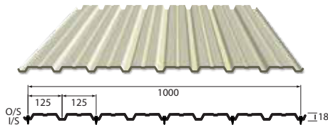
* NordicLiner™ - Liner Panel for Roof & Wall
