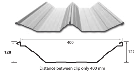
* NordicRoof™ - for Roof Panel
